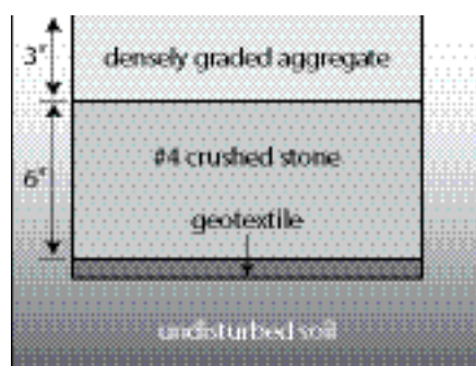
Figure 1. Construction details.
