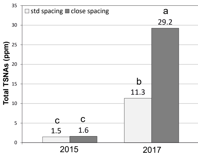
Figure 8. Total TSNA's for a high converter variety cured with standard and close stick spacing, over two years. Bars with different letters are significantly different at the 5% level.
