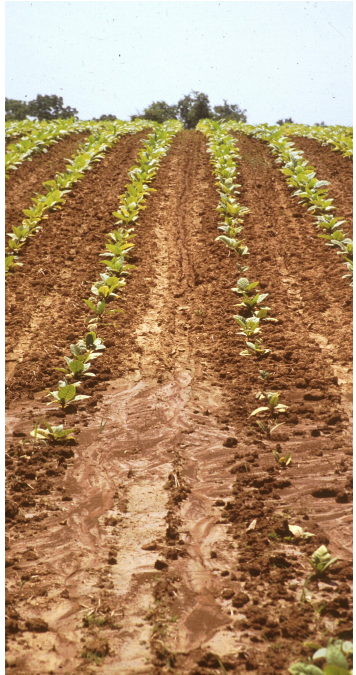
Figure 2. Severe gully erosion in conventionally prepared tobacco field.
