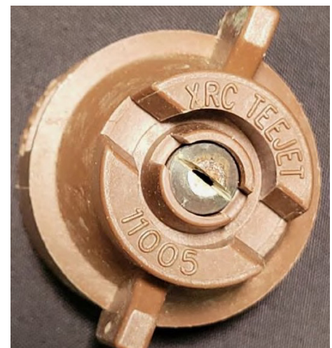
Figure 2. Corroded stainless-steel nozzle tip that should be replaced.
