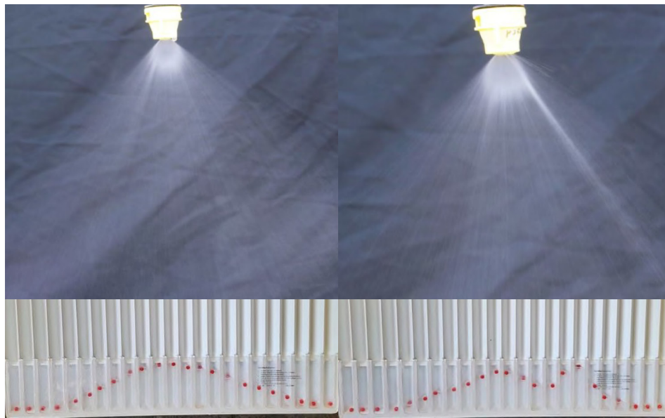
Figure 7. Spray patterns from an 8003 flat-fan, stainless-steel nozzle tip that is in good condition (left) and one that has been damaged by cleaning with metal wire (right). The damage is visible as a heavy stream in the pattern, and it causes a misshapen distribution.
